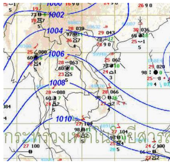
Figure 2: Weather map for 20 th July 2012
