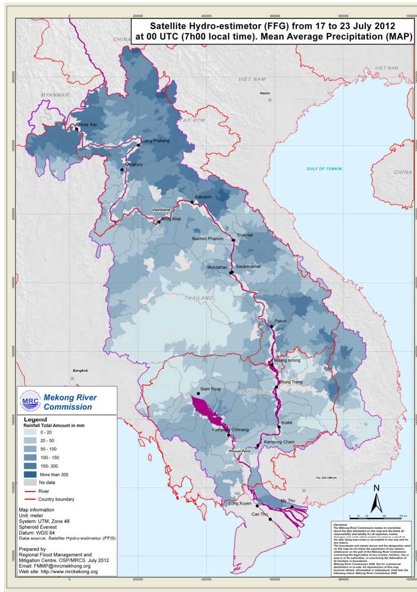
Figure 3: Rainfall distribution over the LMB, from 17 th July to 23 rd July, 2012
