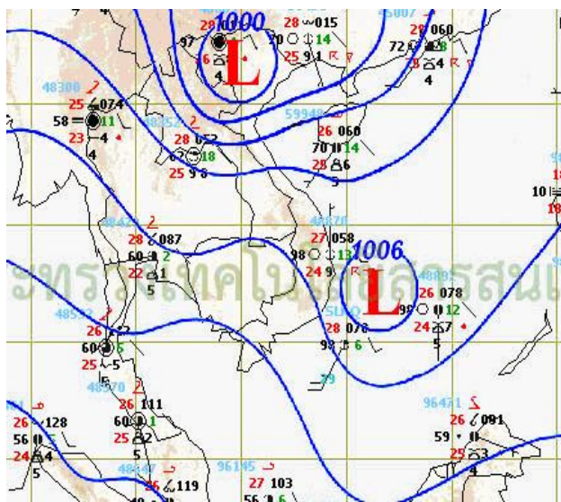
Figure 1: Weather map for 16 th July 2012
